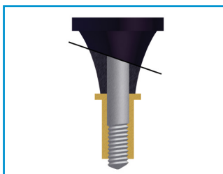
STEP 1 The fastener is threaded onto the pull-up stud of an installation tool.
