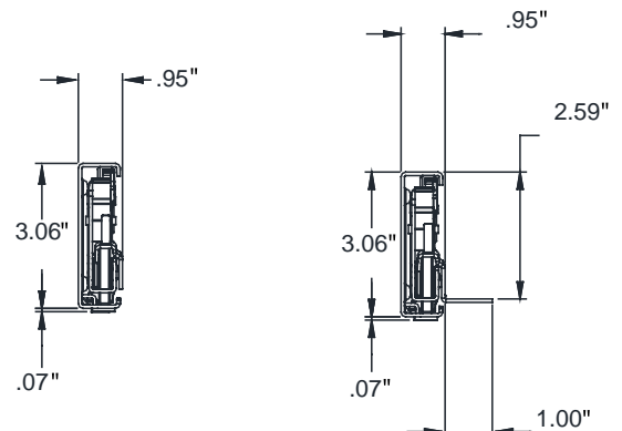
ST8200 Cross Section
